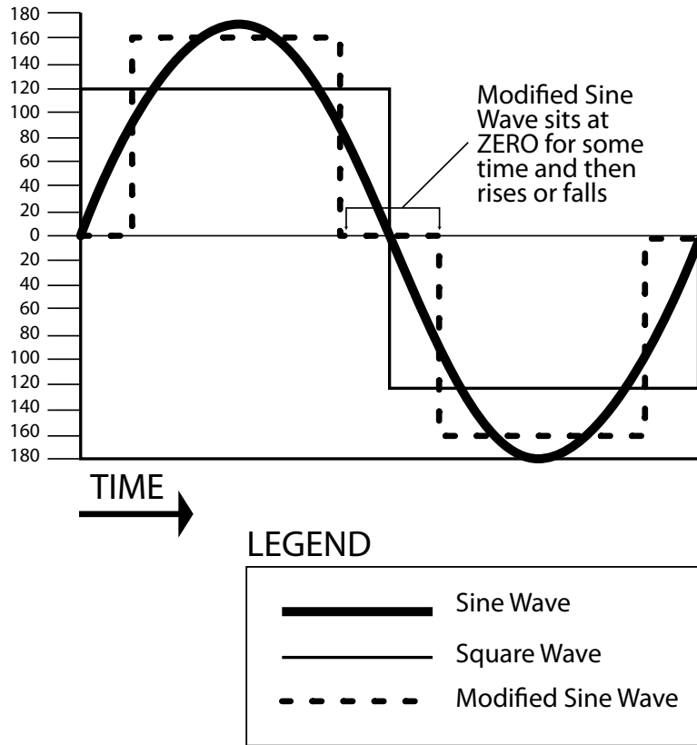
Fig. 1: Square, Modified and Pure Sine Wave
