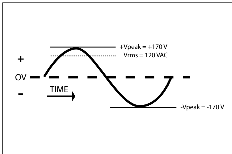
Fig. 2: 120 VAC Sine Wave
