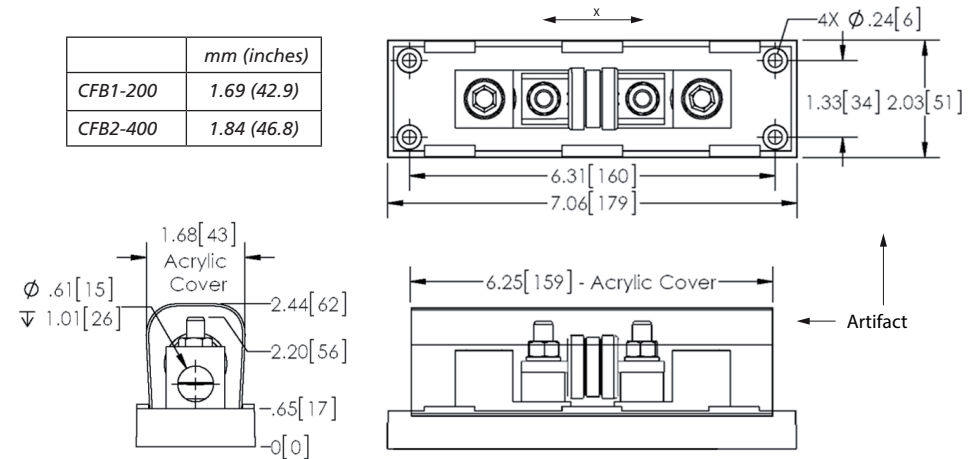
Fig. 5. Fuse Block Dimensions
