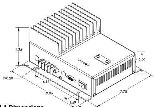
Fig 4.1 Dimensions
