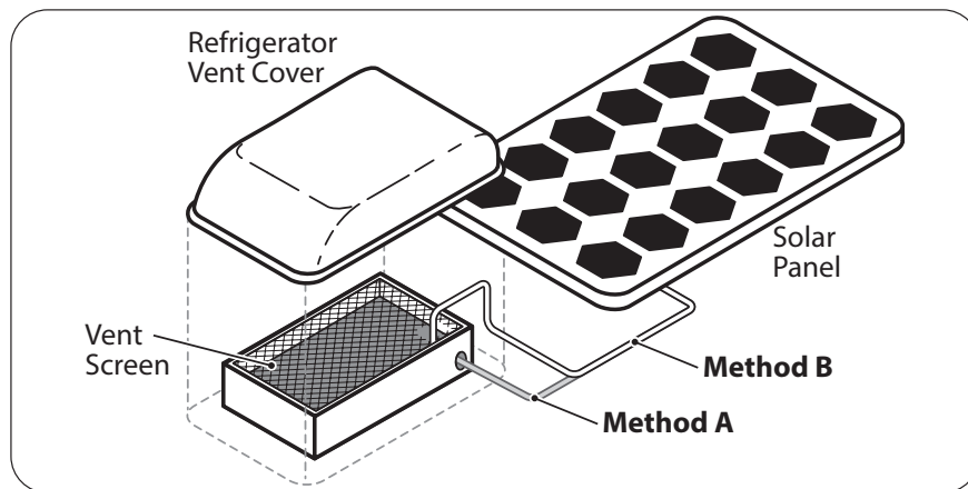
Fig. 4.6 PV Wire Entry Through RV Vent
