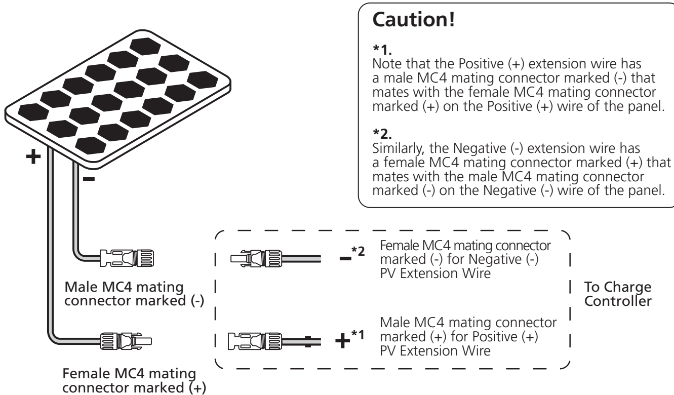
Fig 4.1. Connecting extension wires to the output wires of solar panel
