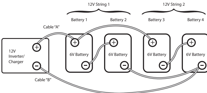
Fig. 4.4 Series-Parallel Connection
