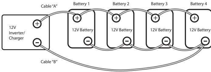
Fig. 4.3 Parallel Connection
